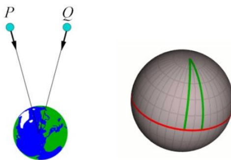
Figure 4: Left: two free-falling particles move along initially parallel paths towards the center of the Earth. There, both paths intersect; right: lines that are initially parallel on the surface of the Earth at the equator, intersect at the North pole.
